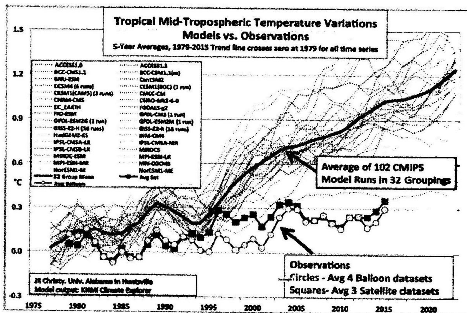
Figure 9 – Average of 102 model runs vs satellite and balloon results (1975-2015)
